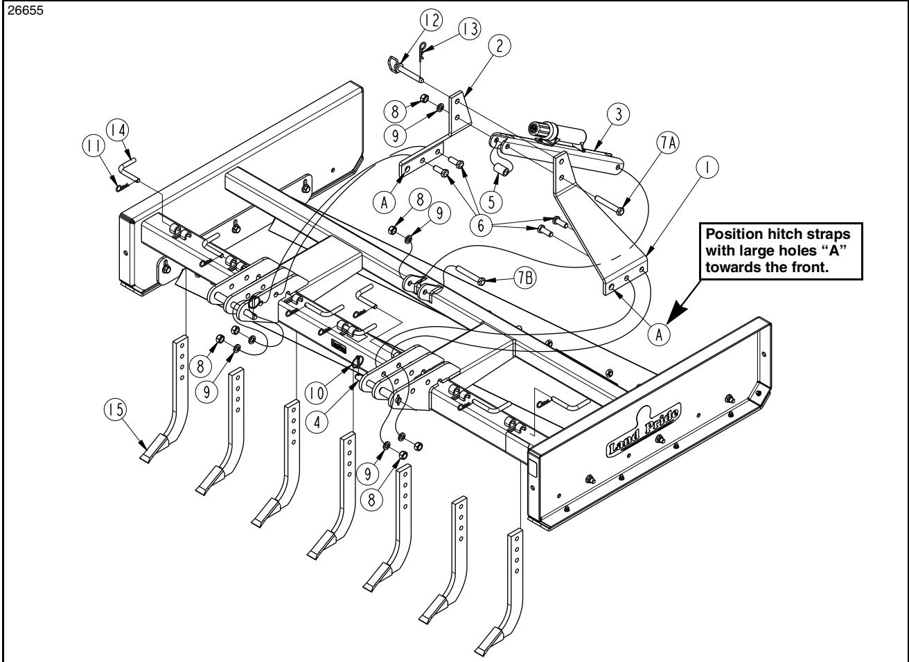
Hitch and Shank Set-up Figure 1-1
