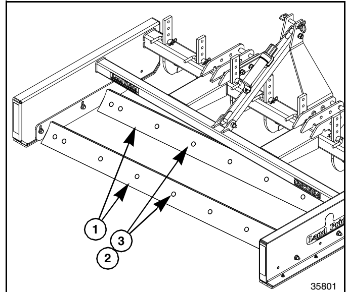
Rear Mounting Cutting Blades Figure 4-2
