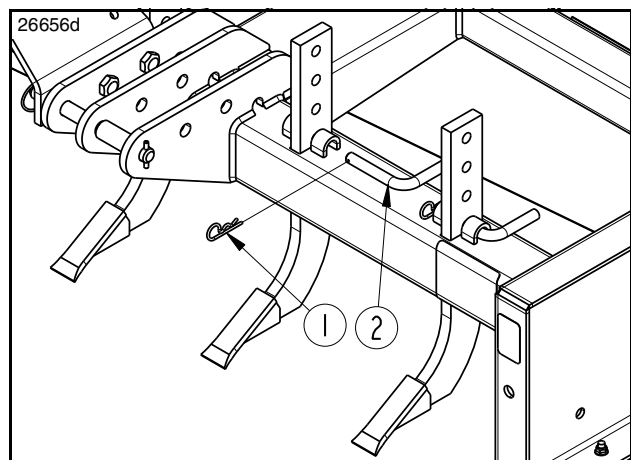
Fourth Hole 2 1/2" (6.4 cm) Above
