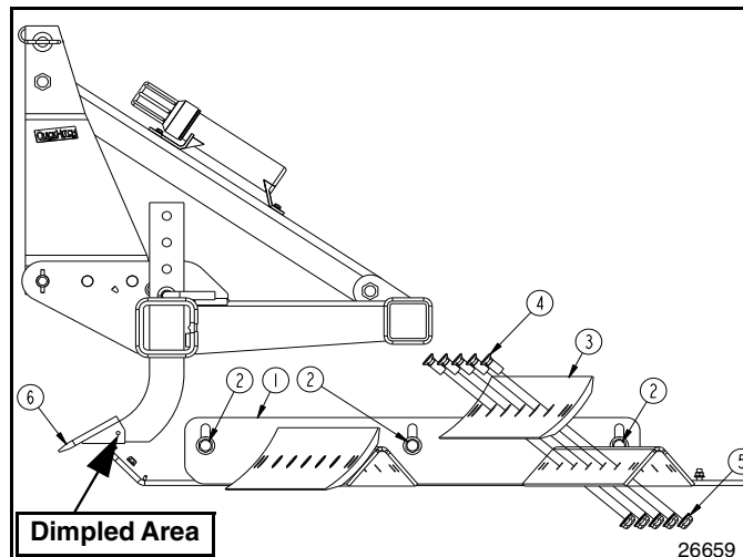
Cutting Blade and Shank Tip Removal Figure 5-1
