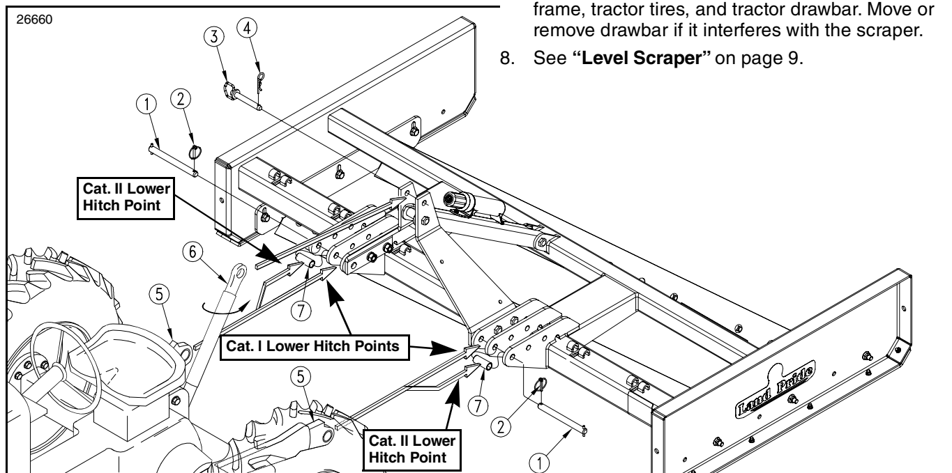
Tractor 3-Point Hitch Figure 1-2
