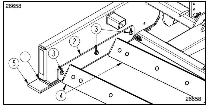
Blade Height Adjustment (Left-Hand Side Shown)
