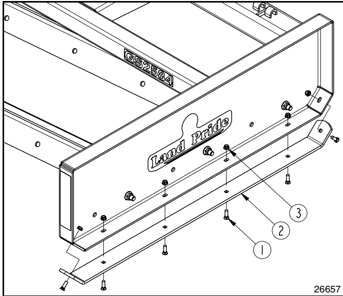
Skid Shoe Maintenance Figure 5-2
