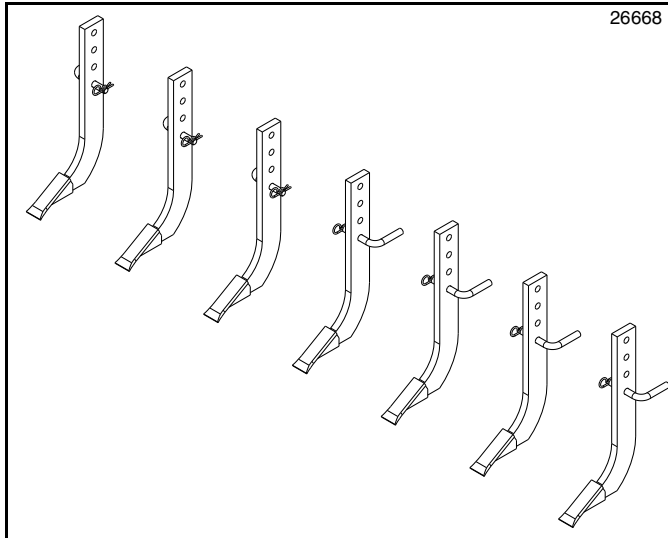
GS2584 - 7 Shank Option Shown Figure 4-1
