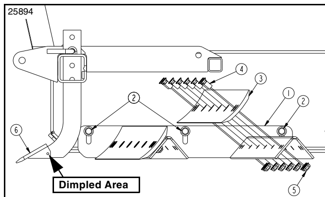
Cutting Blade and Shank Tip Removal Figure 5-1
