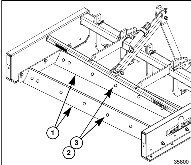
Rear Mounting Cutting Blades
