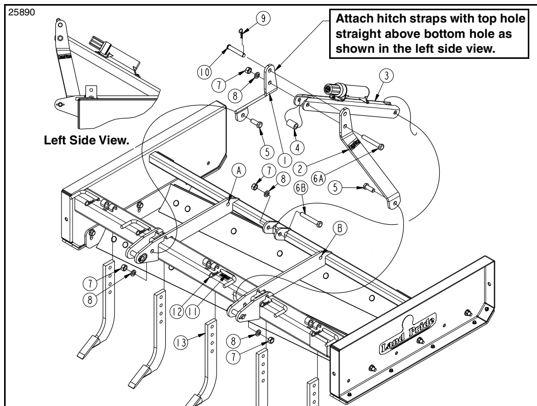
Hitch and Shank Set-up
