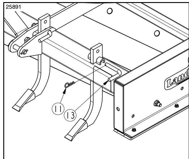
Second Hole 1 1/2" (3.8 cm) Below
