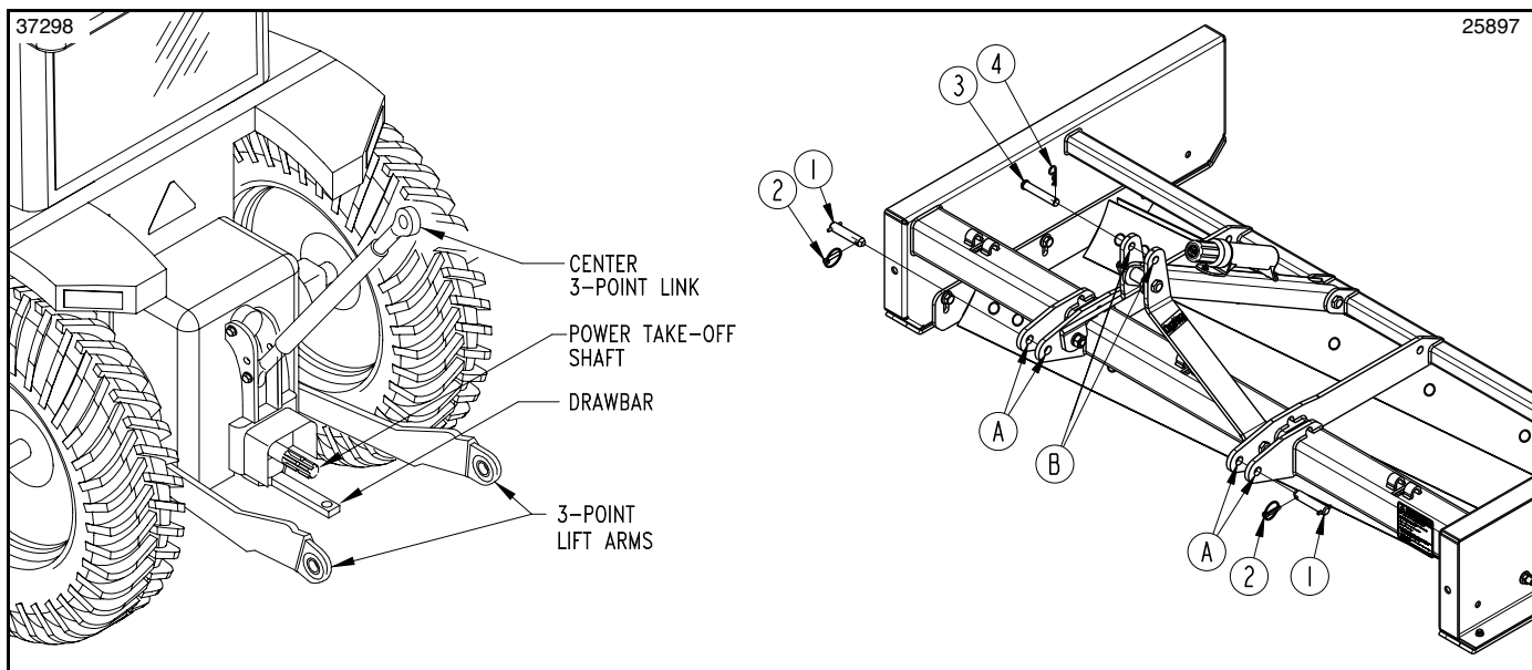
Tractor 3-Point Hitch Figure 1-2
