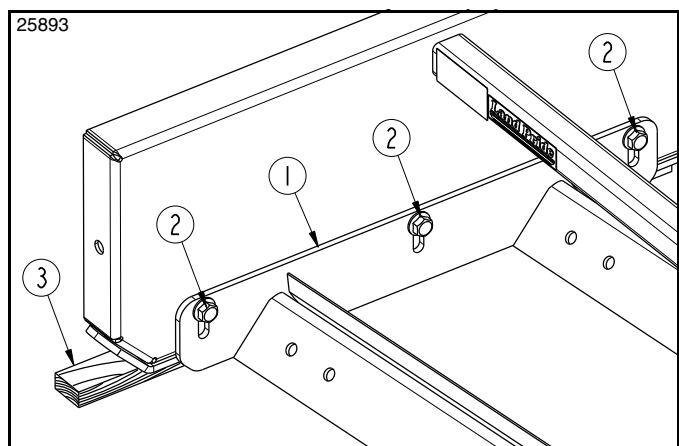
Blade Height Adjustment (Left Side Shown) Figure 2-1
