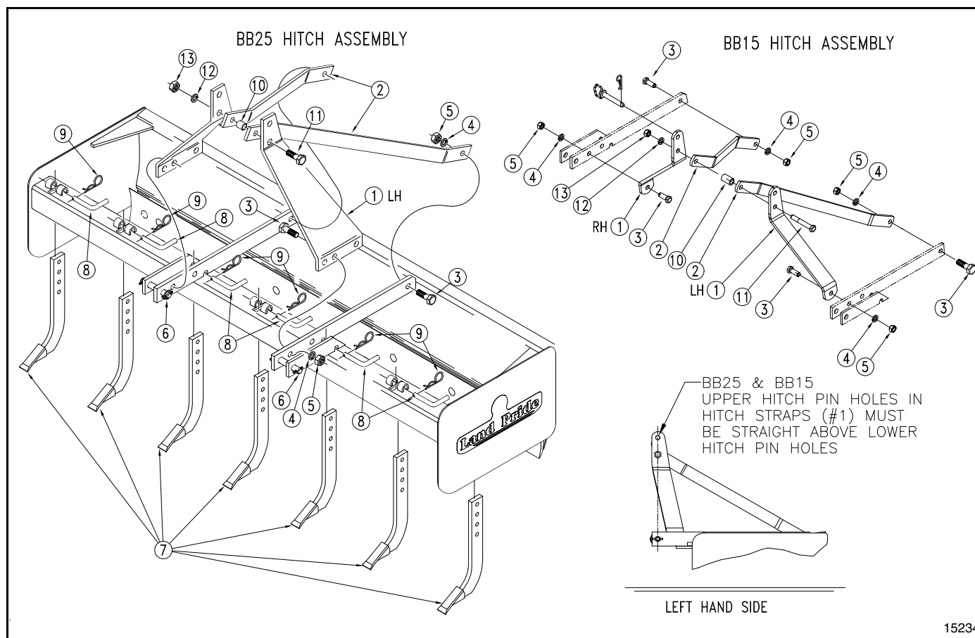
Hitch and Shank Assembly Figure 1-1
