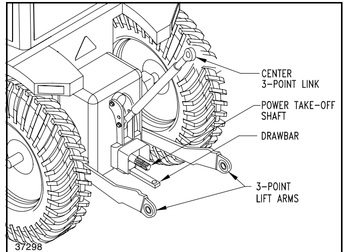
Tractor 3-Point Hitch Figure 1-2
